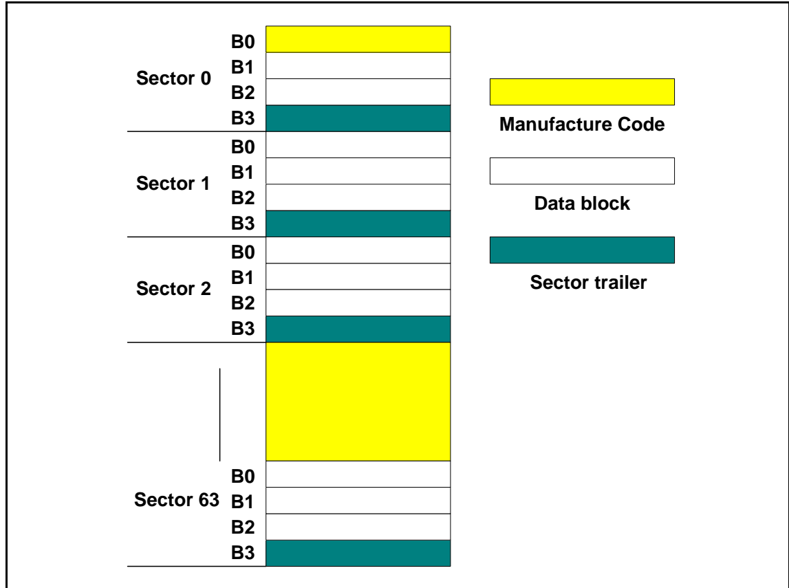
Figure 5-1 FM11RF08SH Memory Organization
