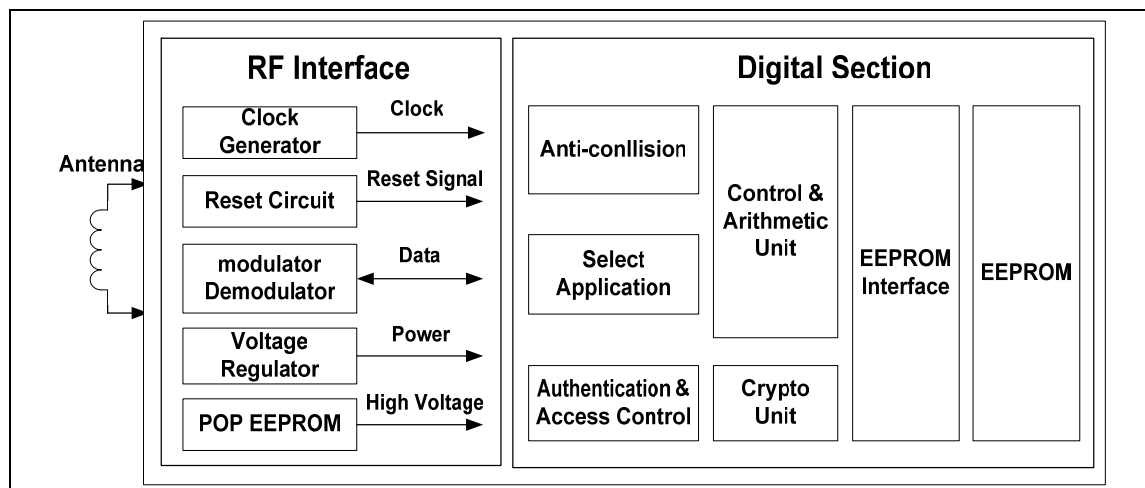
Figure 2-1 FM11RF08SH Block Diagram
