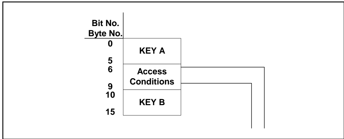
Figure 5-2 FM11RF08SH Structure of Block 3
