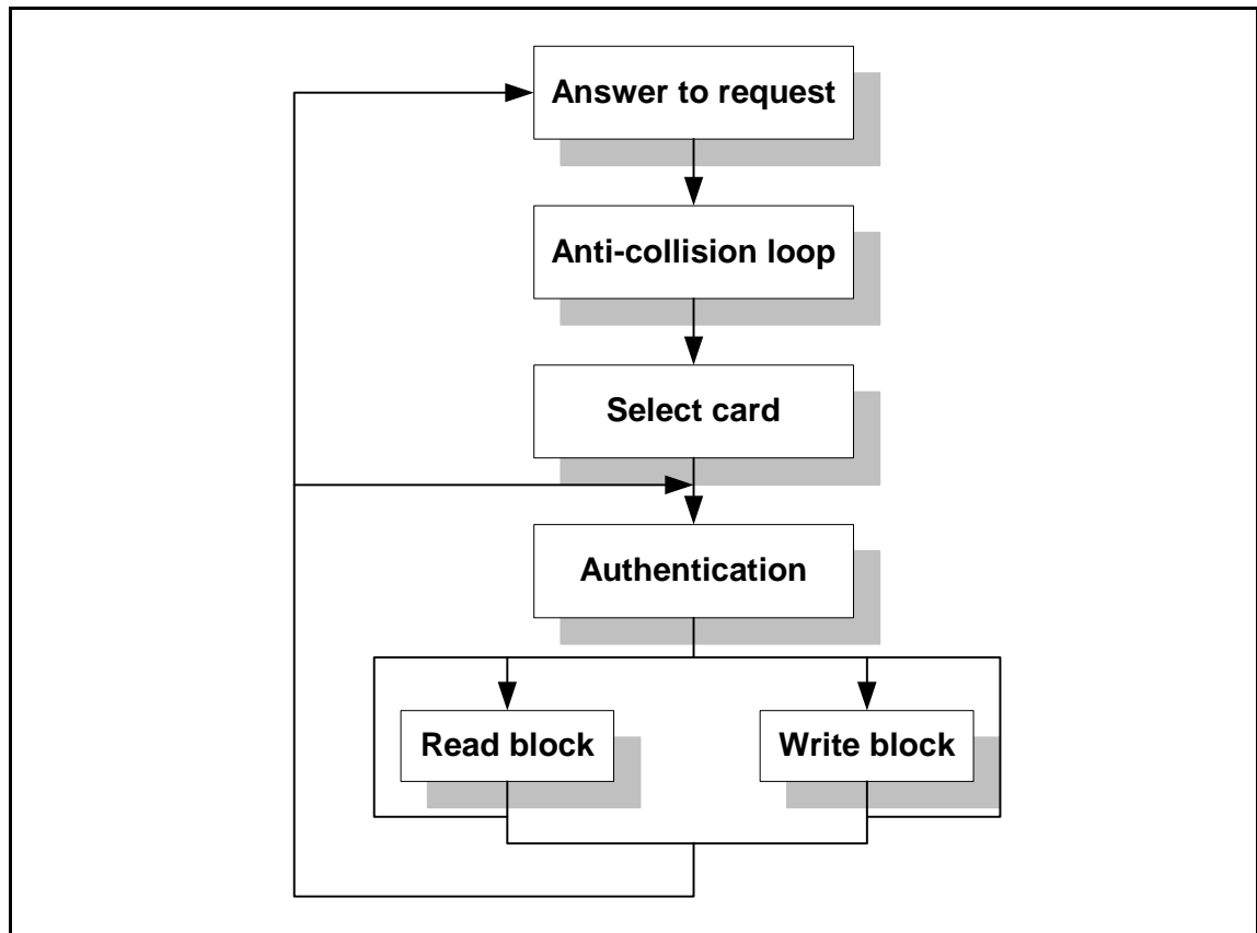
Figure 4-1 FM11RF08SH Transaction Sequence Diagram
